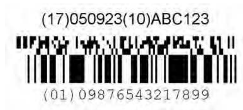
GS1 DataBar Truncated Composite
