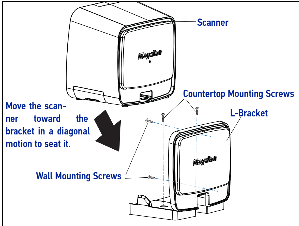
Figure 7. L-Bracket Mount
